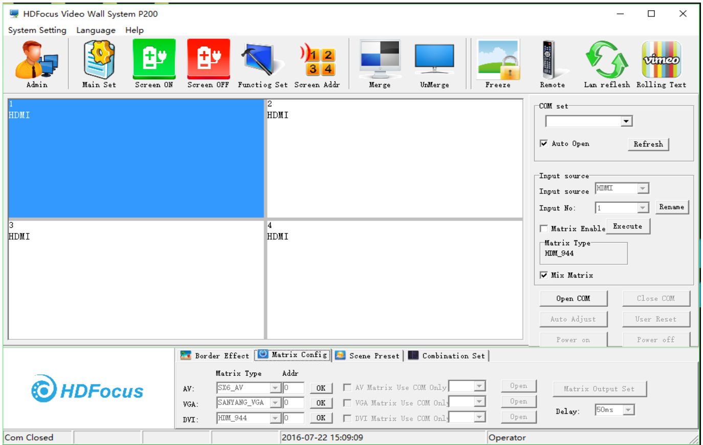
Software Interface
